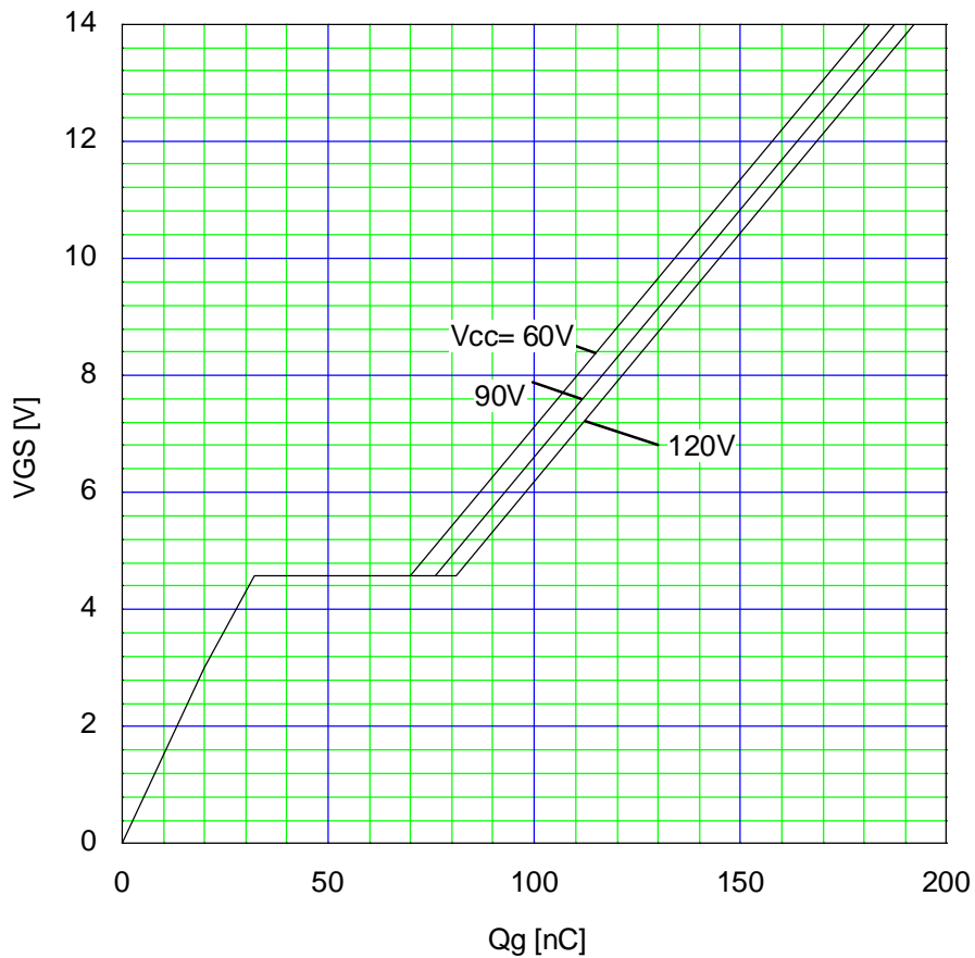
Typical Gate Charge Characteristics V_{GS}=f(Q_g):I_D=65A, T_{ch}=25\text{ }^\circ\text{C}
