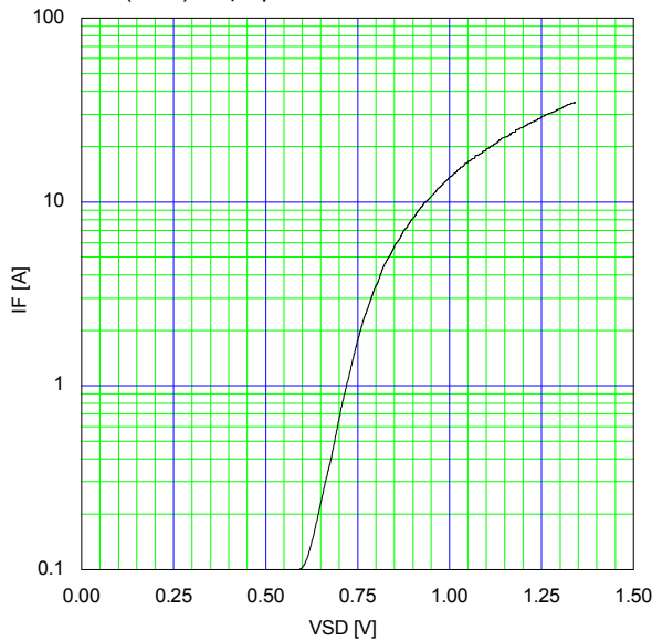
Typical Forward Characteristics of Reverse Diode I_F=f(V_{SD}):80\text{ }\mu s\text{ pulse test}, T_{ch}=25\text{ }^\circ C
