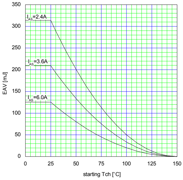
Maximum Avalanche Energy vs. starting Tch E(AV)=f(\text{starting Tch}):V_{CC}=60V, I(AV)\leq 6A
