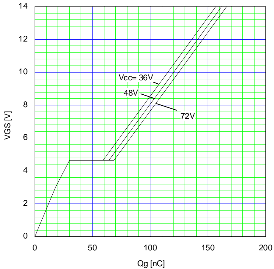
Typical Gate Charge Characteristics V_{GS}=f(Q_g):I_D=80A,T_{ch}=25\text{ }^\circ\text{C}
