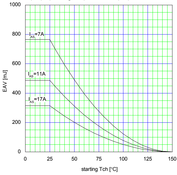
Maximum Avalanche Energy vs. starting Tch E(AV)=f(\text{starting Tch}):V_{CC}=60V, I(AV)\leq 17A
