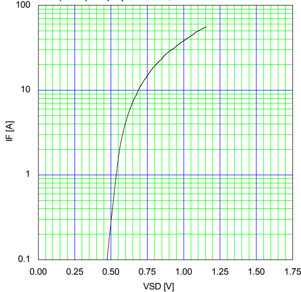
Typical Forward Characteristics of Reverse Diode I_F=f(V_{SD}):80\ \mu\text{s pulse test}, T_{ch}=25\text{ }^\circ\text{C}
