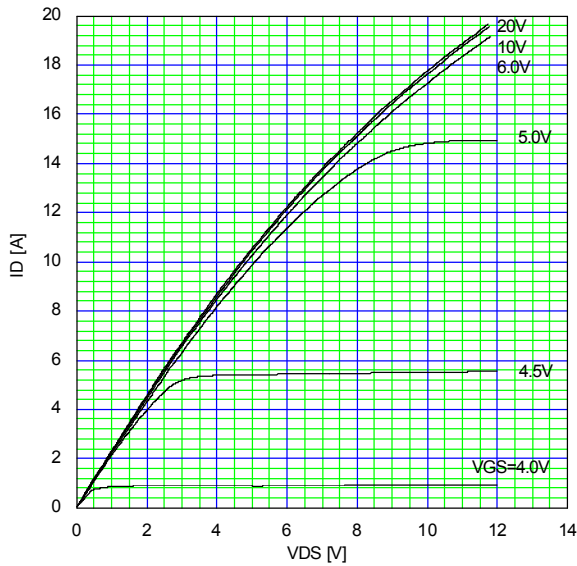
Typical Output Characteristics I_D=f(V_{DS}):80\mu\text{s pulse test},T_{ch}=25^\circ\text{C}
