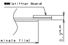
コネクタ接続部詳細 (導通面) Connector (Conductive face)
