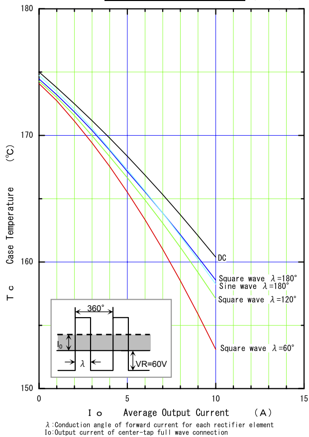
Current Derating (Io-To) (max.)
