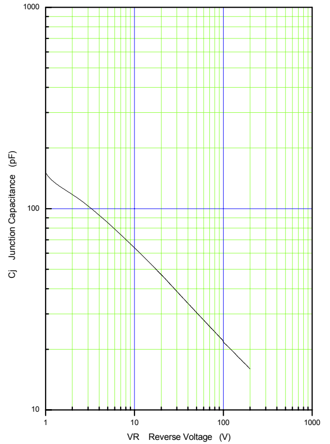
Junction Capacitance Characteristic (max.)
